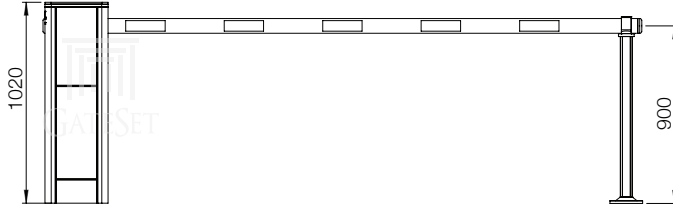
Barrier Side View
